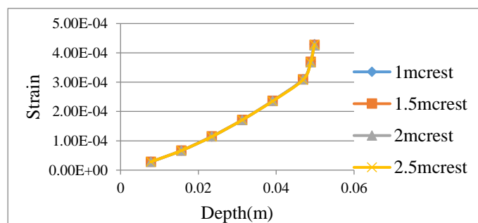
Fig.17.Strain vs Depth
