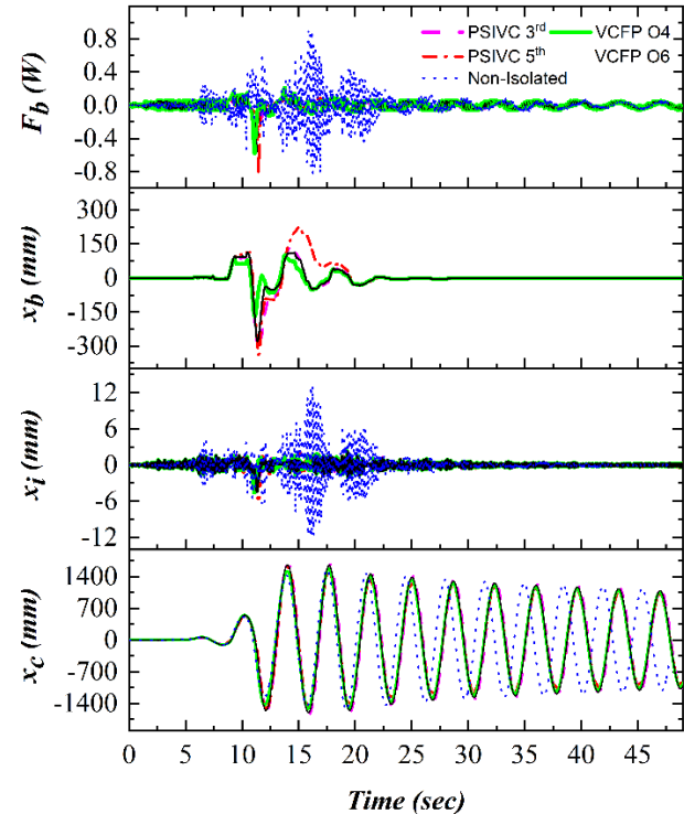
Figure 12 Variations with respect to time of base shear, impulsive, isolator & sloshing displacement of slender tank for Landers ground excitation, 1992 (Lucerne Valley)
