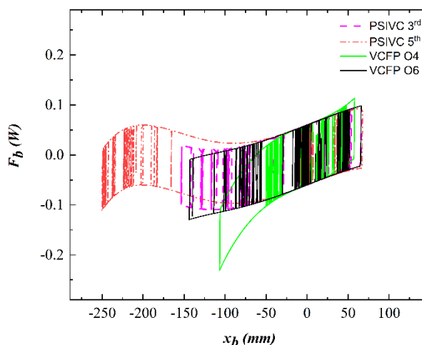
Figure 6 Bearing displacement variation of base shear for broad tank with isolators mentioned above for Landers ground excitation, 1992 (Lucerne Valley)
