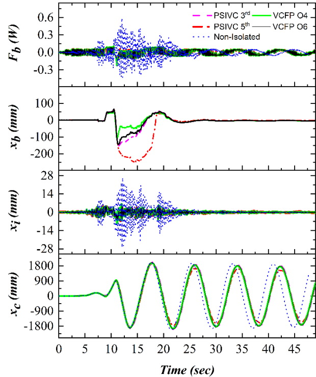
Figure 8 Variations with respect to time of base shear, impulsive, isolator & sloshing displacement of broad tank for Landers ground excitation, 1992 (Lucerne Valley).
