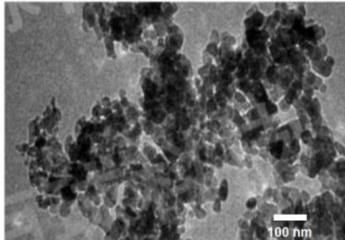
Figure 2. TEM image of \text{Al}_2\text{O}_3 nanoparticles [18]
